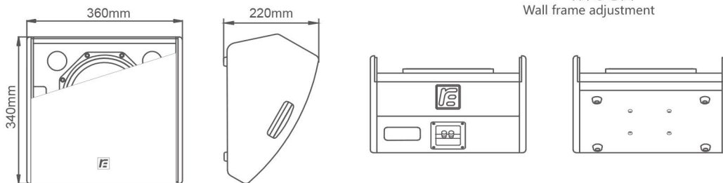
M8R墙架示意图 Wall frame adjustment
